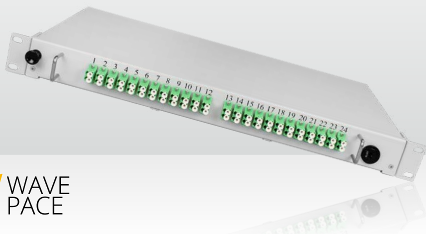
10443957 SP-48-Pull-Panel-LC/APC
